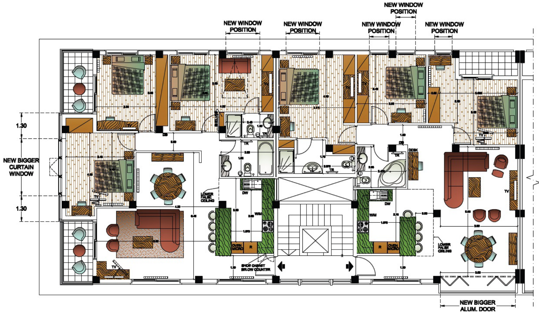
Typical Floor
